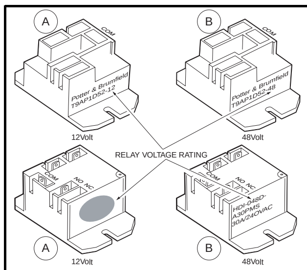
Figure 1 Verify Relay Voltage Rating
